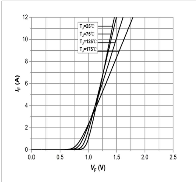
Figure 1: Forward Characteristics
