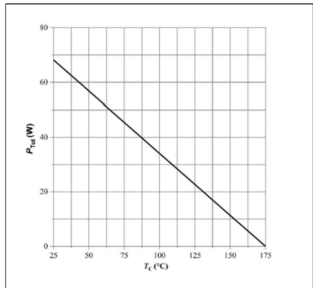
Figure 4: Power Derating
