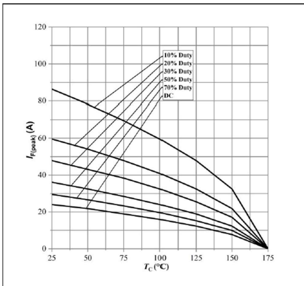
Figure 3: Current Derating
