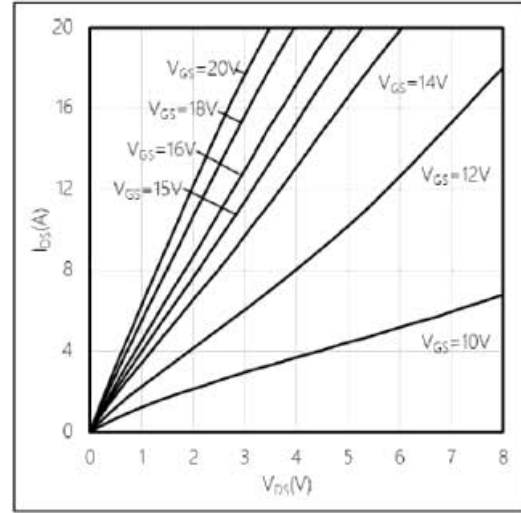
Figure 2. Typical Output Characteristics T_j = 25^{\circ}\text{C}
