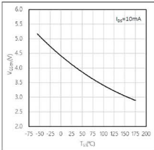
Figure 11. Threshold Voltage vs. Temperature
