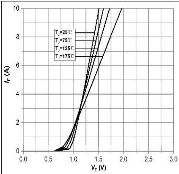
Figure 1: Forward Characteristics
